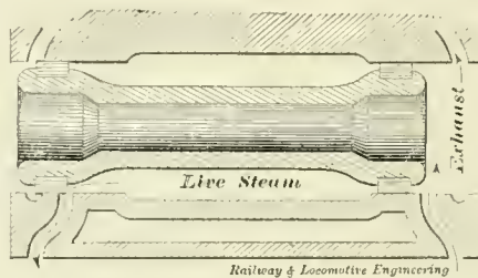
FIG. 8. CENTRAL ADMISSION PARTLY OPENED.
